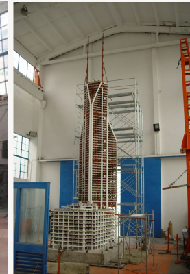
Model tests on shaking table
